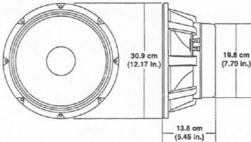
FIGURE 5 — Dimensions
