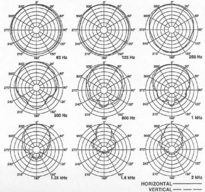
FIGURE 9 — Polar Response
