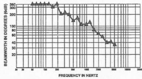
FIGURE 8 — Directivity vs. Frequency
