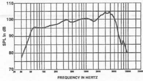
FIGURE 1 — Axial Response in Typical Enclosure (2.0 ft 3 ), 1 Wa/1 Meter
